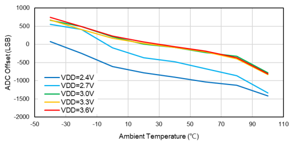
Figure 11 ADC Offset vs. Temperature
