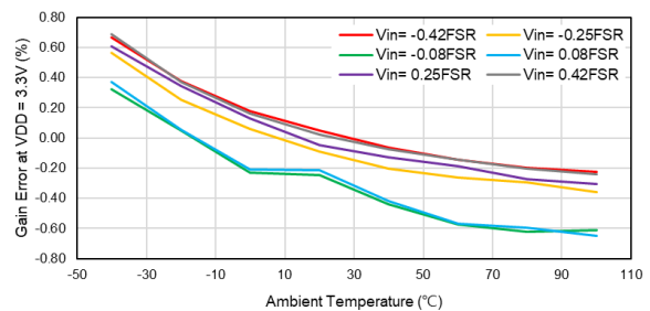
Figure 12 Gain Error vs. Temperature
